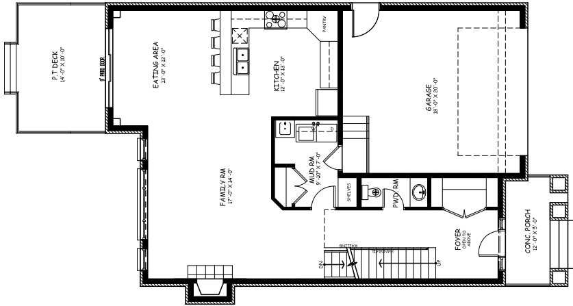
GROUND FLOOR PLAN E & O.E
